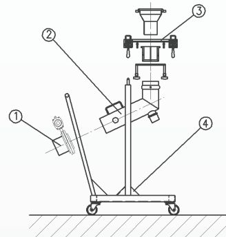
Systemtube
