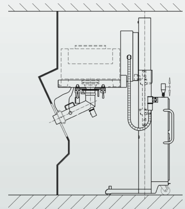
emptying position
