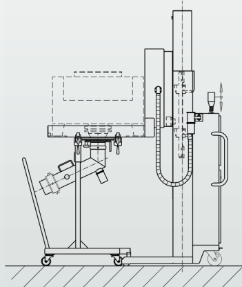
pick-up position for the systemtube
